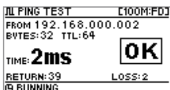
Ping test
